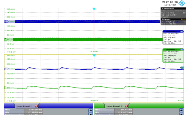
Figure 47 – Output Ripple Voltage Waveforms. 265 VAC Input. 5 V_{PK} : 14 mV, 12 V_{PK} : 34 mV. Upper: 5 V, 20 mV / div. Lower: 12 V, 40 mV / , 10 ms, 20 \mu s / div.
