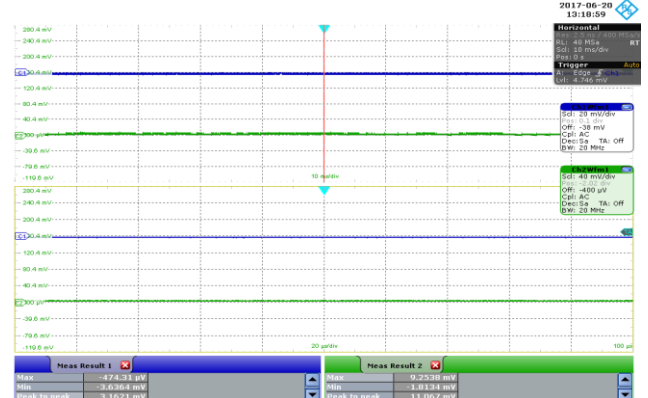
Figure 45 – Output Ripple Voltage Waveforms. 265 VAC Input. 5 V_{PK} : 4 mV, 12 V_{PK} : 12 mV. Upper: 5 V, 20 mV / div. Lower: 12 V, 40 mV / , 10 ms, 20 \mu s / div.
