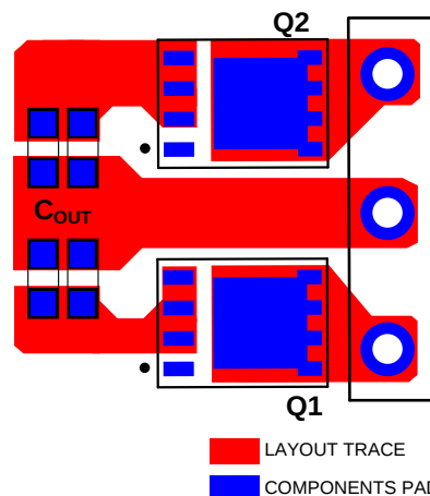
Figure 14: Layout Example for System Power Loop
