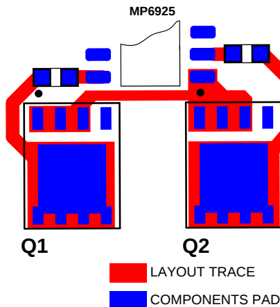
Figure 8: Layout Example for Sensing Loop and V_{DD} Decoupling
