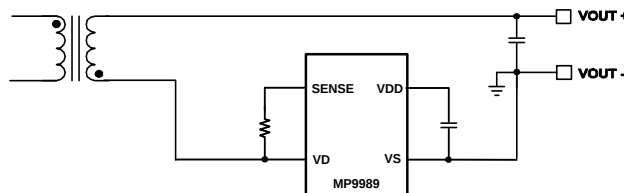
Figure 3: Low-Side Rectification
