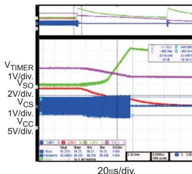
Over-Current Protection
