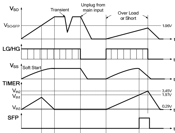
Figure 37: SFP Timing
