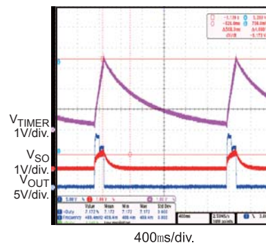
Start-Up Failure Protection SO Pin Open
