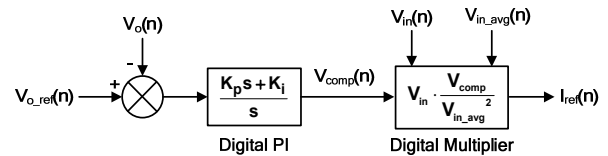
Figure 17: Current Reference
