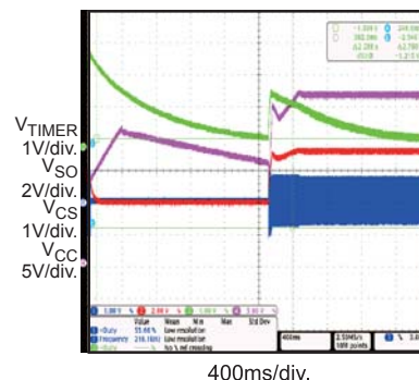
Over-Current Protection Recovery
