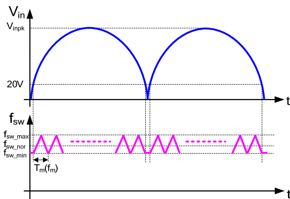
Figure 27: Frequency Jittering
