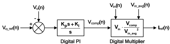
Figure 20: Current Reference
