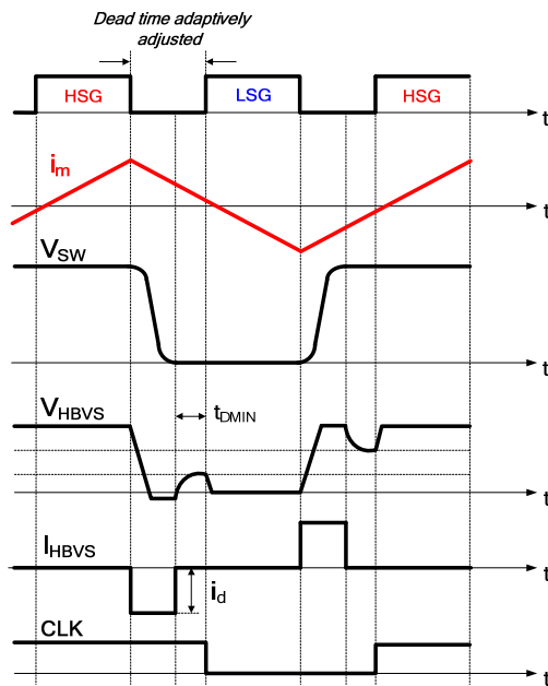
Figure 31: Operation Waveform of ADTA
