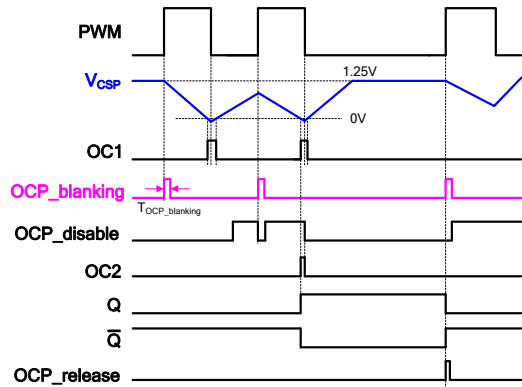
Figure 15: OCP Operation Waveform
