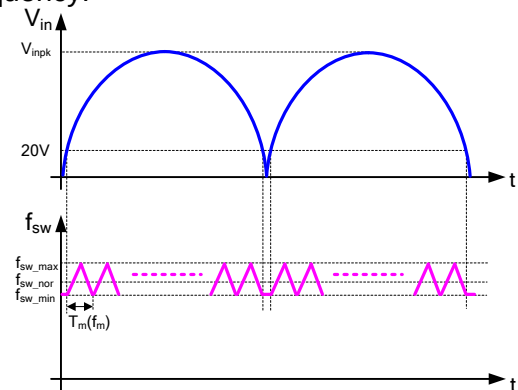
Figure 22: Frequency Jittering
