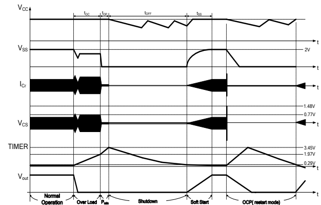
Figure 30: OCR Timing Sequence
