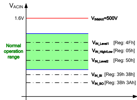
Figure 9: Input Voltage Level for Different Functions
