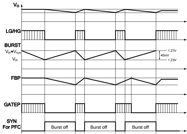
Figure 34: Burst-Mode Operation
