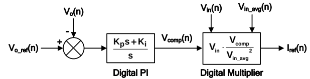
Figure 17: Current Reference
