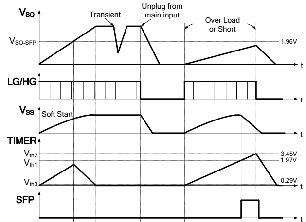
Figure 35: SFP Timing
