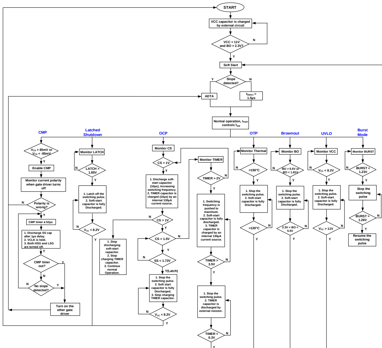
Figure 27: Control Flowchart
